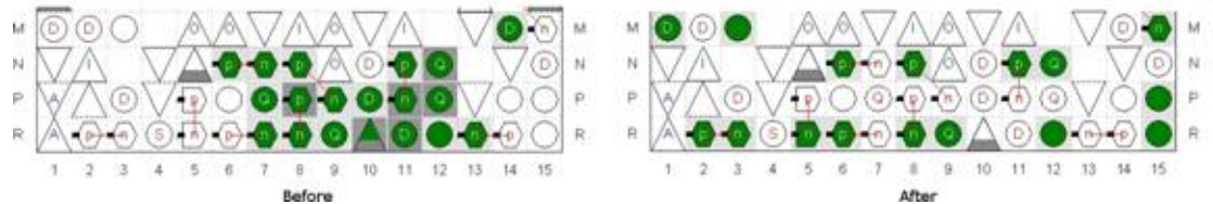
Figure 8. SSN Analysis Results Before and After Using the SSN Optimization Logic Option
