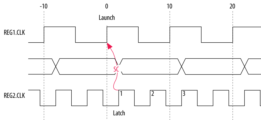
Figure 93. Setup Timing Diagram
