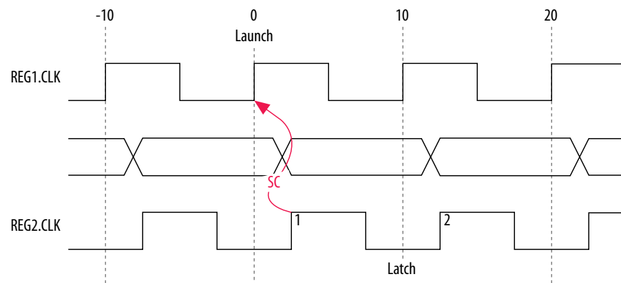
Figure 80. Setup Timing Diagram
