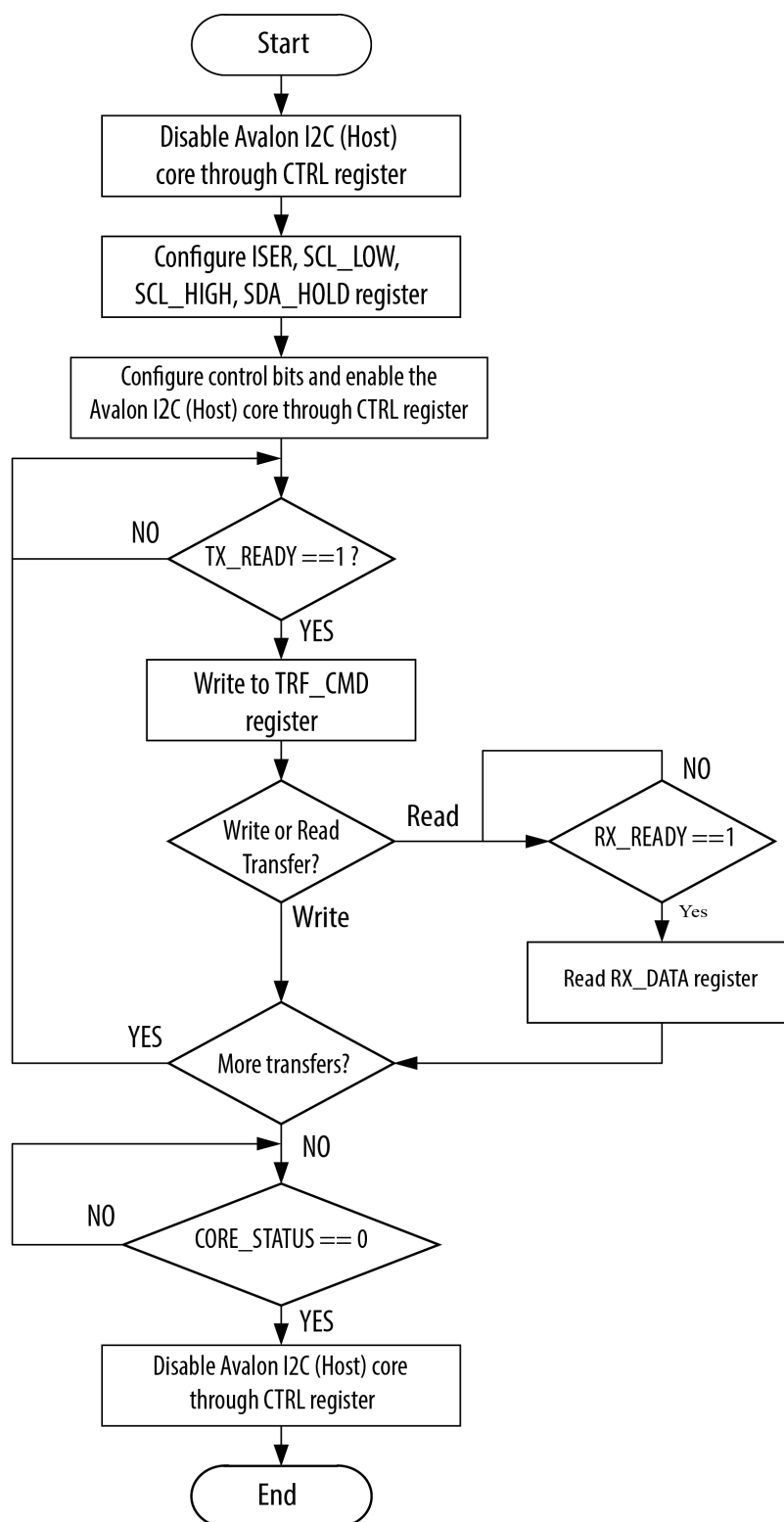
Figure 55. Programming Model Flowchart
