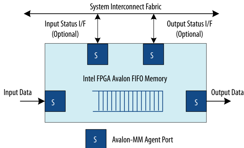
Figure 74. FIFO with Avalon-MM Input and Output Interfaces
