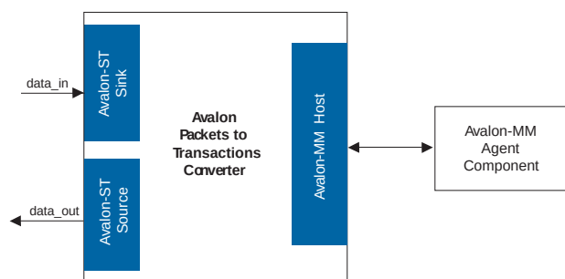
Figure 148. Avalon Packets to Transactions Converter Core
