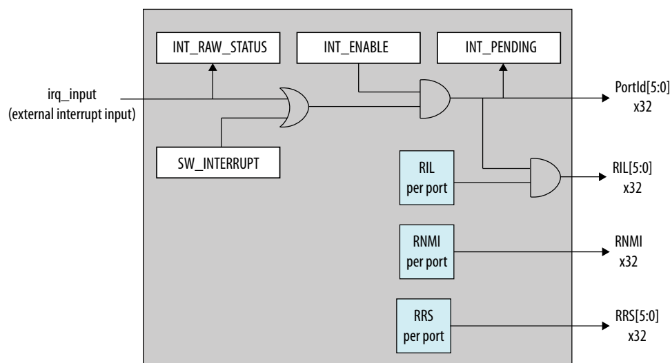
Figure 135. Interrupt Request Block
