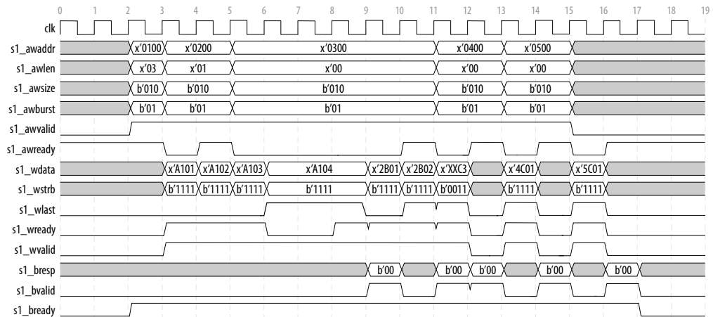
Figure 93. AXI Write with Back Pressure (WVALID back pressure)
