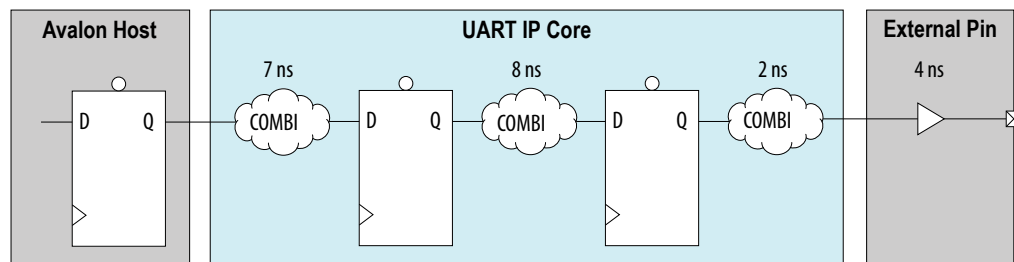
Figure 35. Maximum Delays on UART
