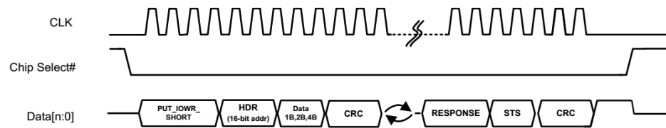
Figure 25. eSPI Host Initiated Short I/O Write Transaction
