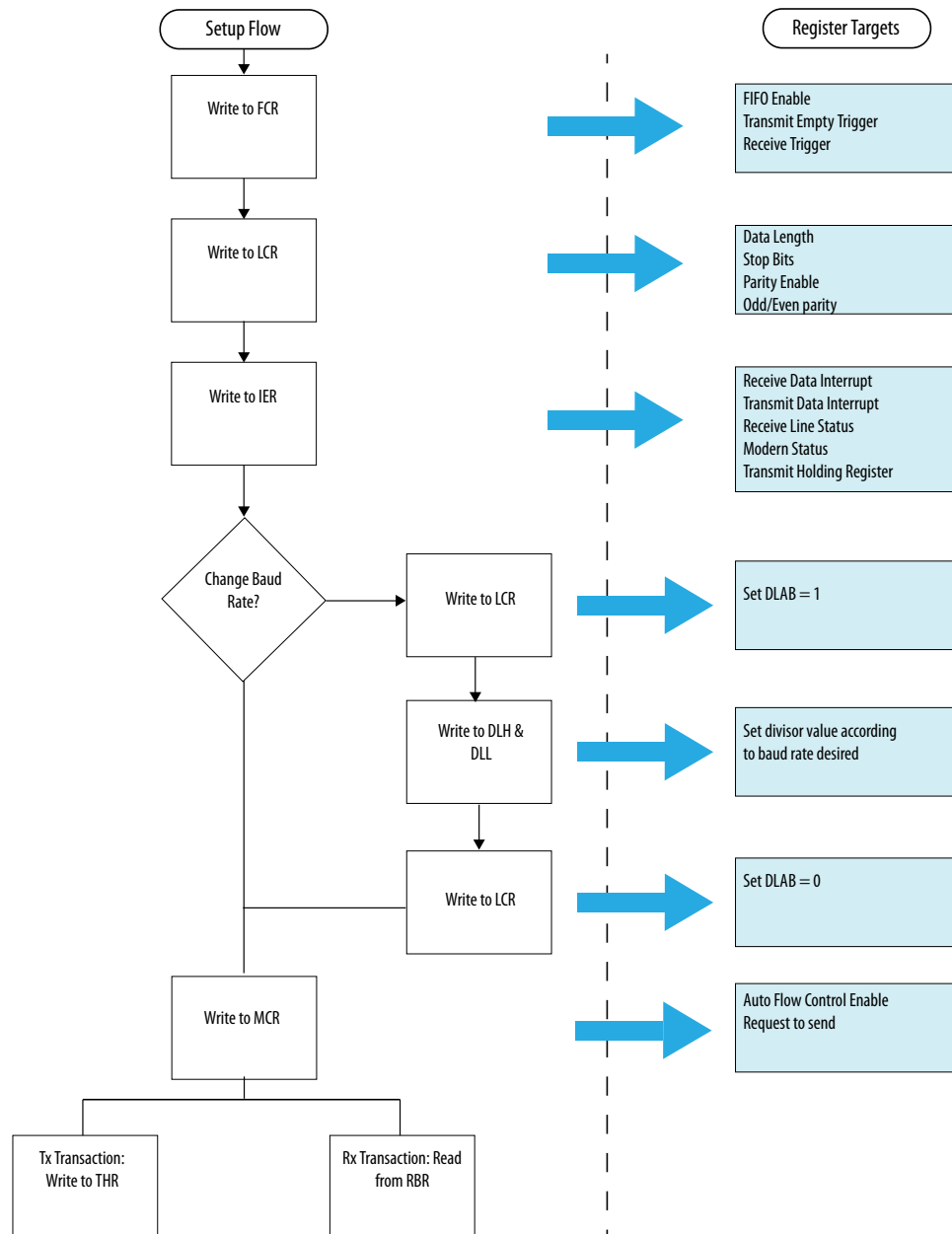
Figure 33. 16550 UART Configuration Flow
