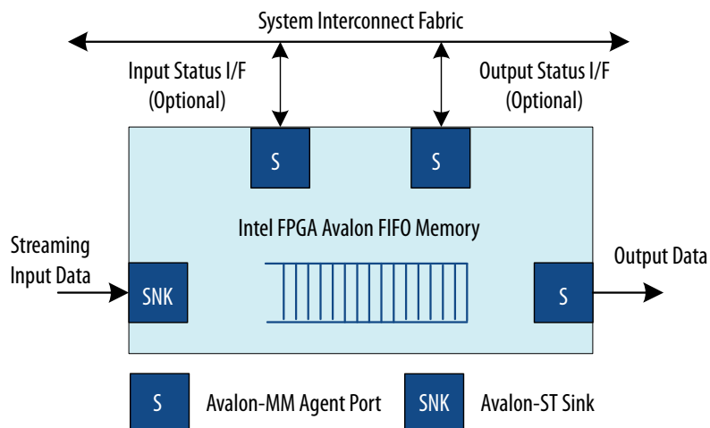
Figure 77. FIFO with Avalon-ST Input and Avalon-MM Output
