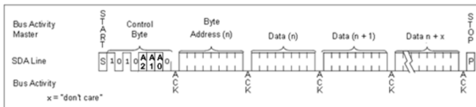
Figure 61. Write Operation
