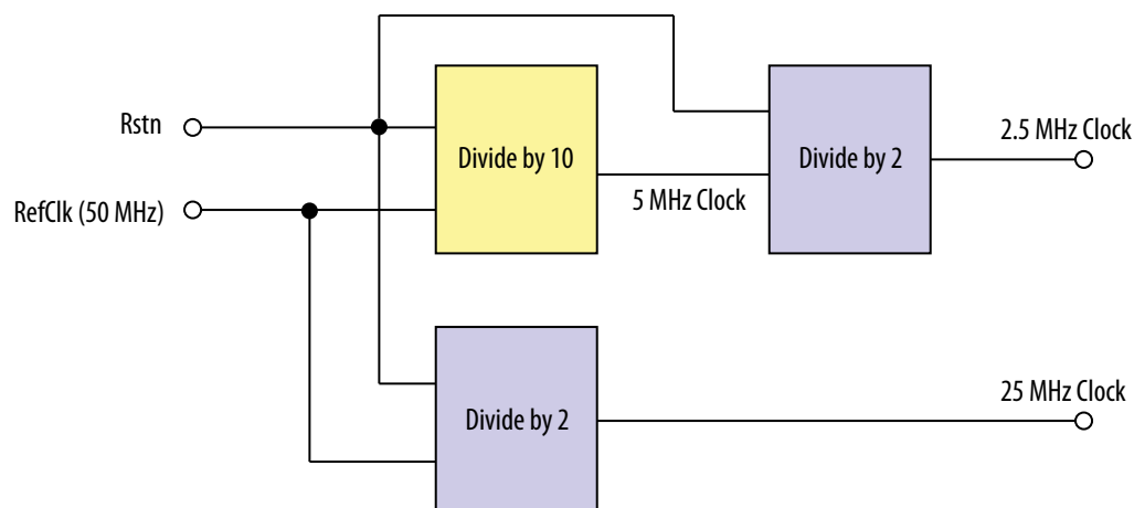
Figure 169. Clocking Scheme
