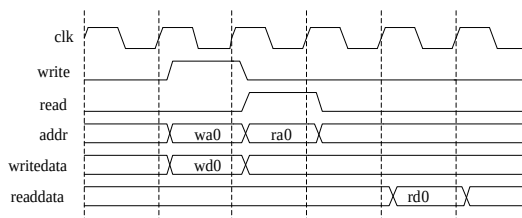
Figure 54. Write and Read Timing of Avalon-MM Agent Interface
