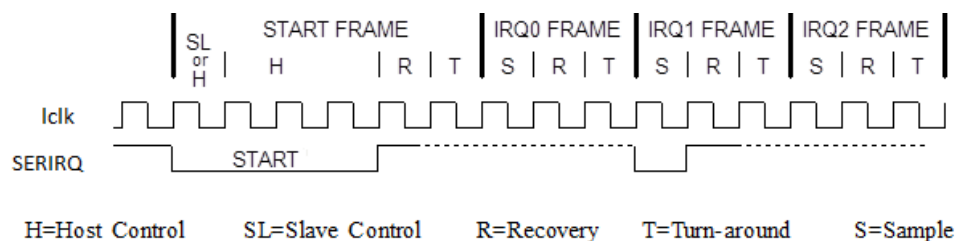
Figure 29. SERIRQ Event Timing Diagram
