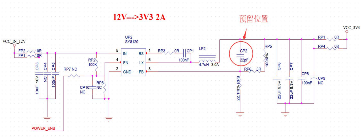
Figure 12 DC-DC step-down circuit diagram
