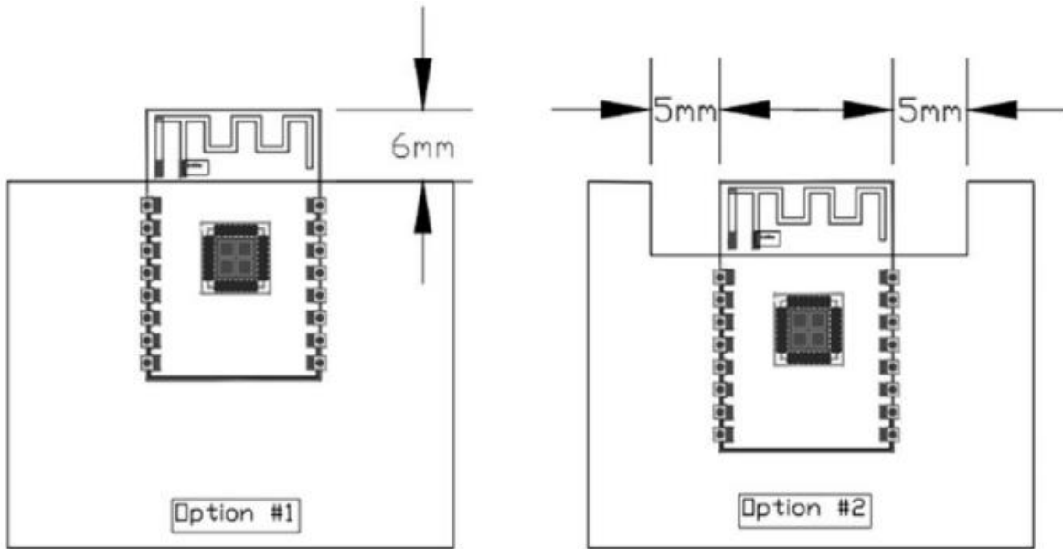
Figure 11 Schematic diagram of antenna layout
